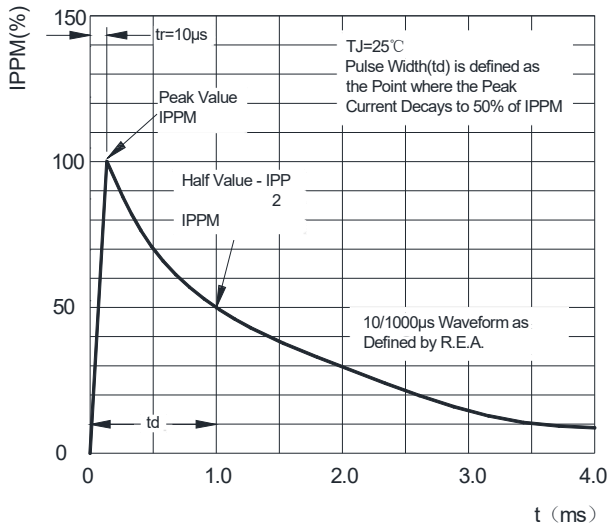
FIG3: Pulse Waveform
